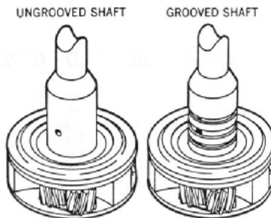
FIG. 10 OUTPUT SHAFT VARIATIONS
